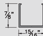
Channel Sill Interior Application Only • Not Thermally Broken
