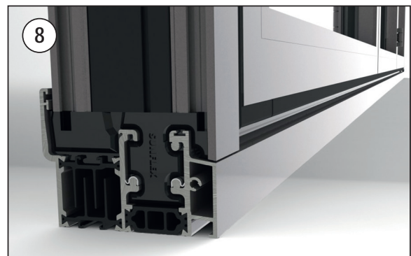
Assembly shoes allow a fast assembly and precise adjustment of the vertical frame profiles
