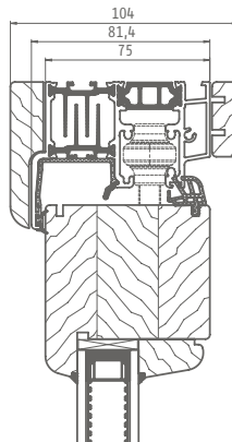
Top rail
