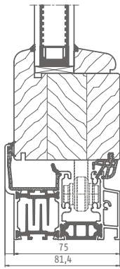
Bottom rail
