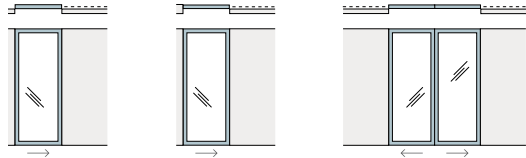
Single Sliding
