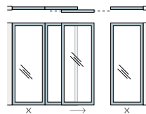
Demountable (Fixed) Panel with Slider
