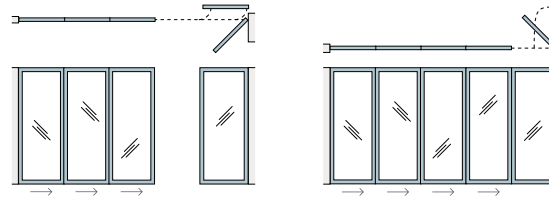
Stacking Wall with Pivot
