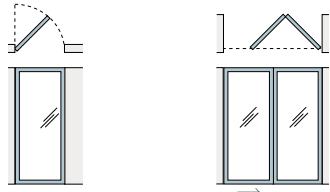
Swinging (Pivot) Folding End
