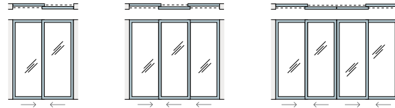
Sliding Bypass
