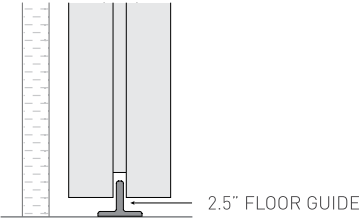
Single Sliding
